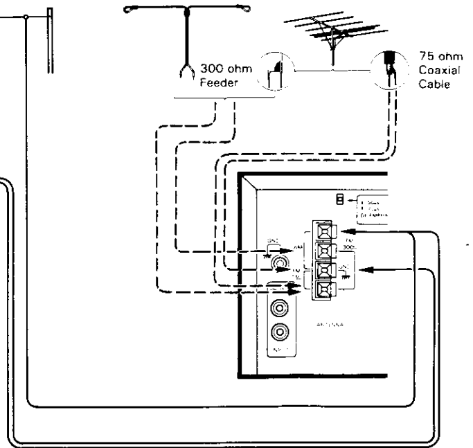
AM outdoor antenna
